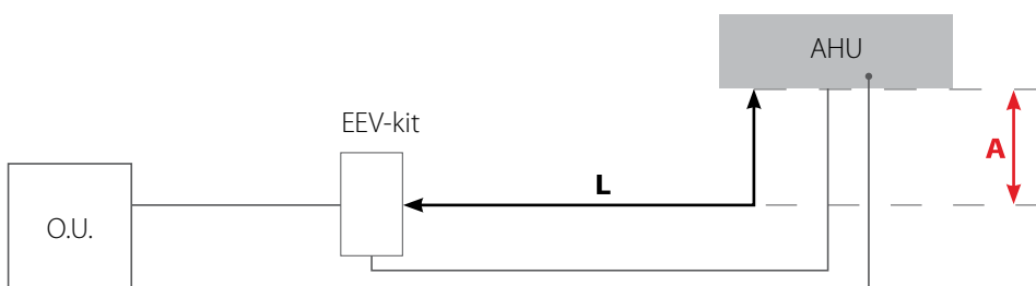
The EEV-kit must be installed in a vertical position 90 ± 15°
